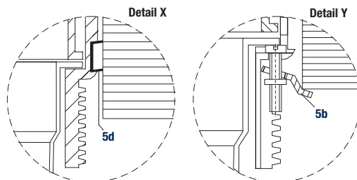
Detail X
