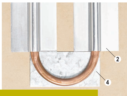
Wand-Heiz-Kühlelement WHK-GK
