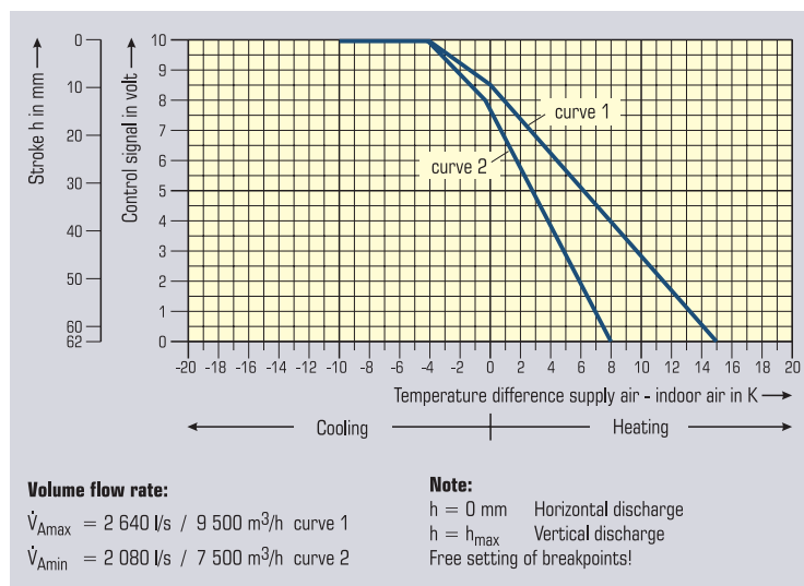
Controller performance chart (example)
