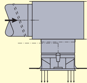
Temperature difference control device, type ST-E
