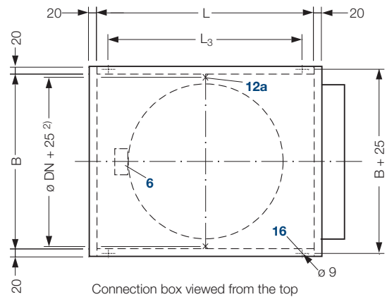
Connection to connection box
