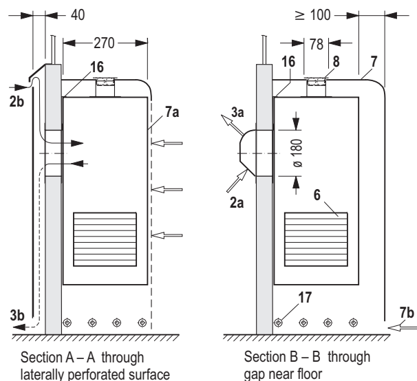
Figure 1: Main dimensions and view of return air vents in the client's parapet covering. The figure also shows an example of the concealed intake/discharge apertures ( 2b and 3b ) and the visible type 2a and 3a ; water connection right 18 , control unit and mains connection 19
