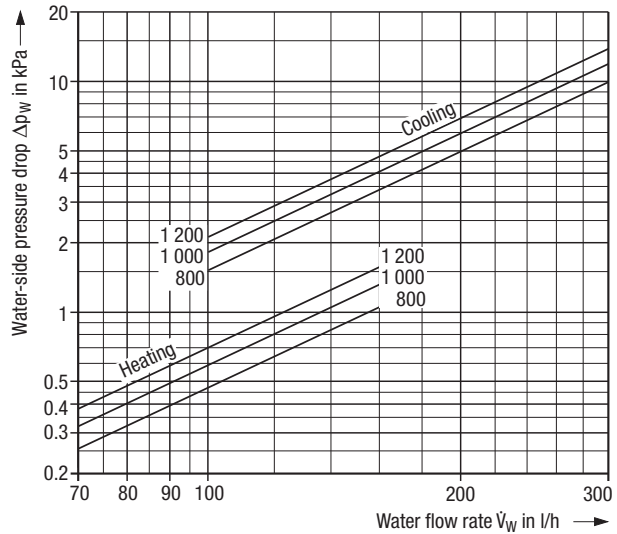
Graph 6: Water-side pressure drop of heat exchanger
