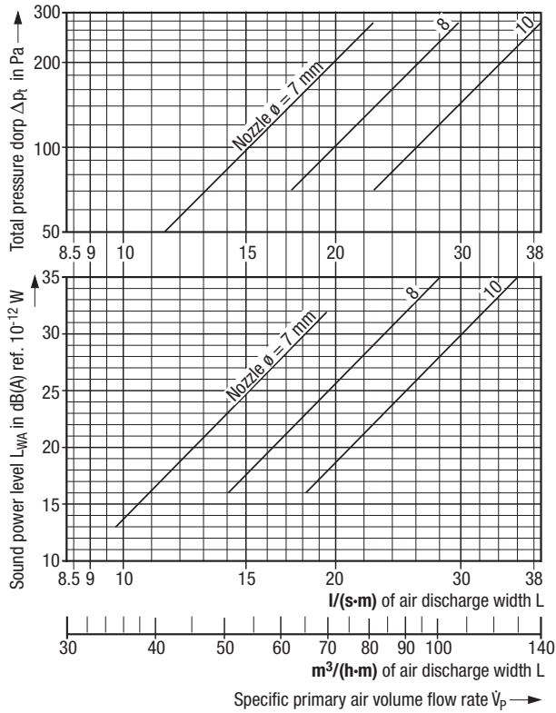
Graph 5: Sound power level and primary air-side pressure drop
