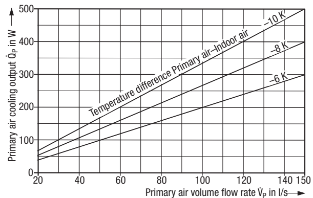
Graph 2: Primary air-side cooling output
