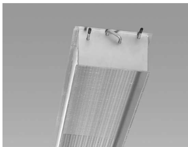
Figure 3: Installation of DK-FZ chilled beam above a pervious false ceiling
