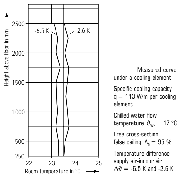
Figure 8: Vertical temperature gradient; cooling ceiling (SKS system) and ceiling twist outlets
