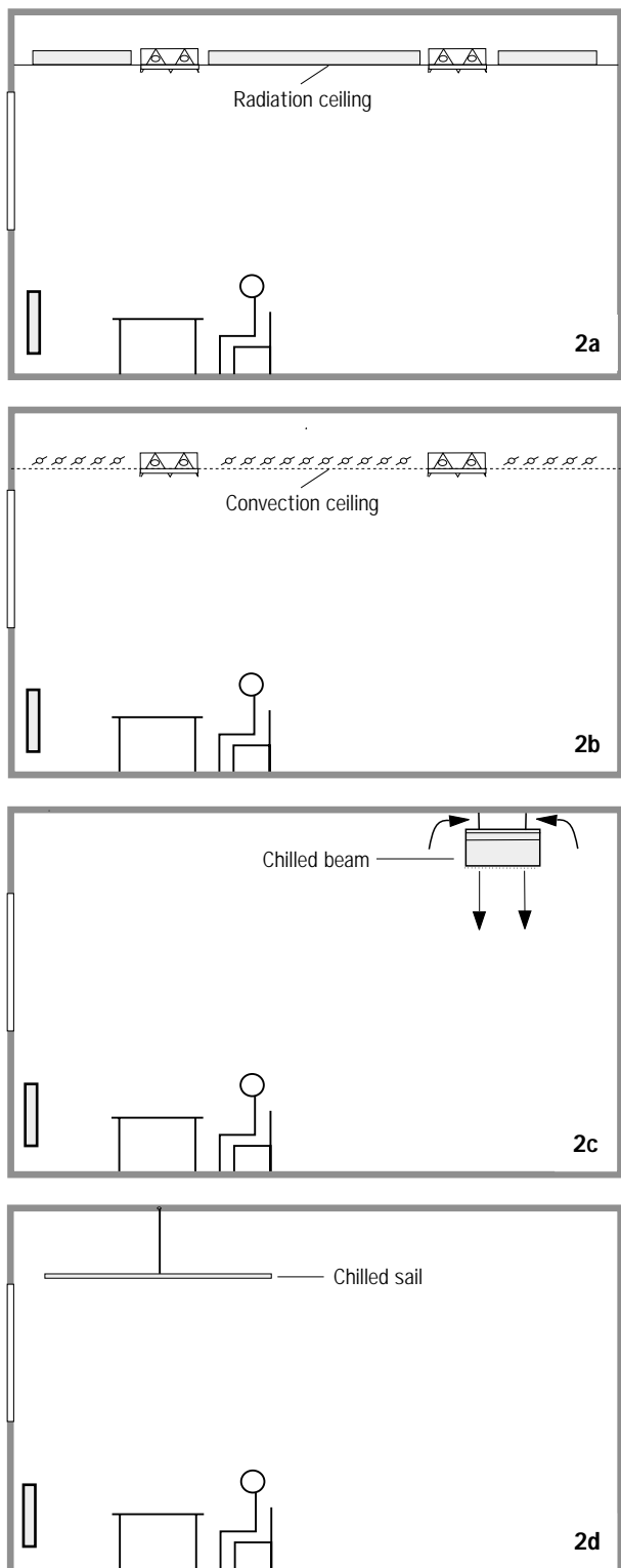
Figure 2: Placement of different cooling ceilings 2a: Large-surface cooling ceiling as radiation ceiling 2b: Large-surface cooling ceiling as convection ceiling 2c: Chilled beam 2d: Chilled sail
